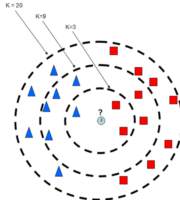
K-Nearest Neighbour
