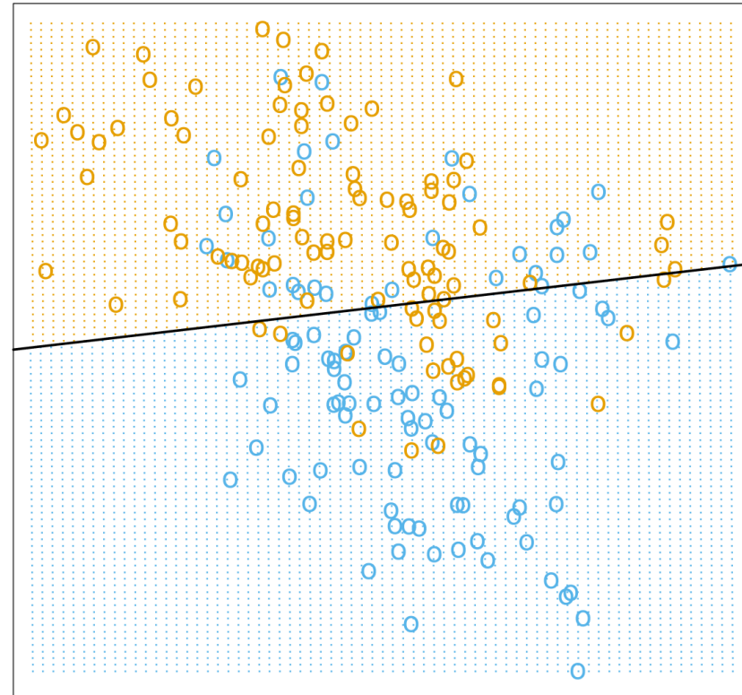
Linear Regression of 0/1 Response
